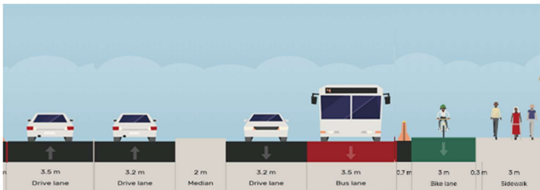
Option 3 - Hutt Road Indicative Cross Section
