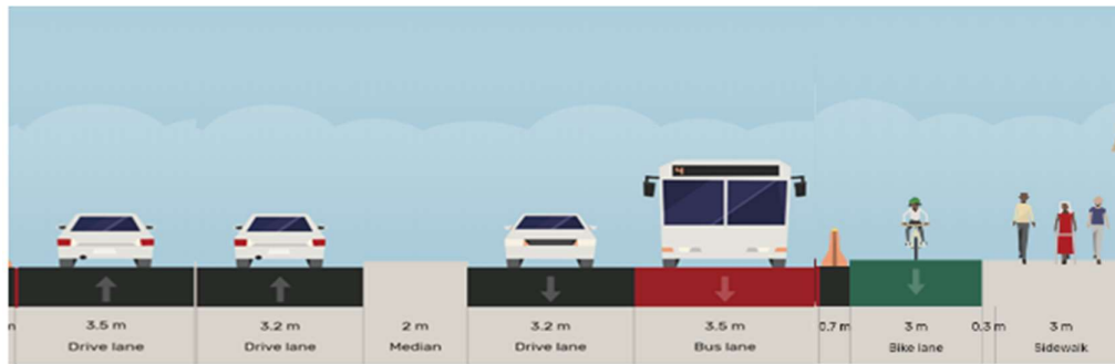
Option 1 - Hutt Road Indicative Cross Section
