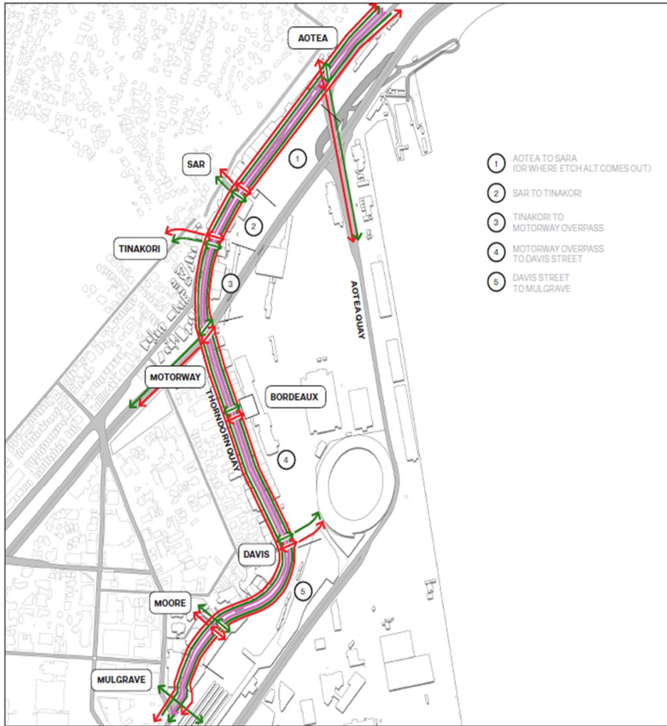
Option 2 - Thorndon Quay Indicative Plan
