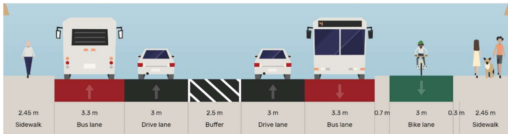
Option 4 - Thorndon Quay Indicative Cross Section
