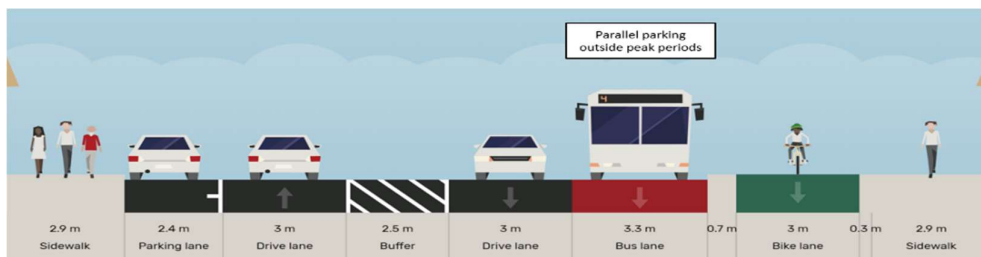
Option 1 - Thorndon Quay Indicative Cross Section
