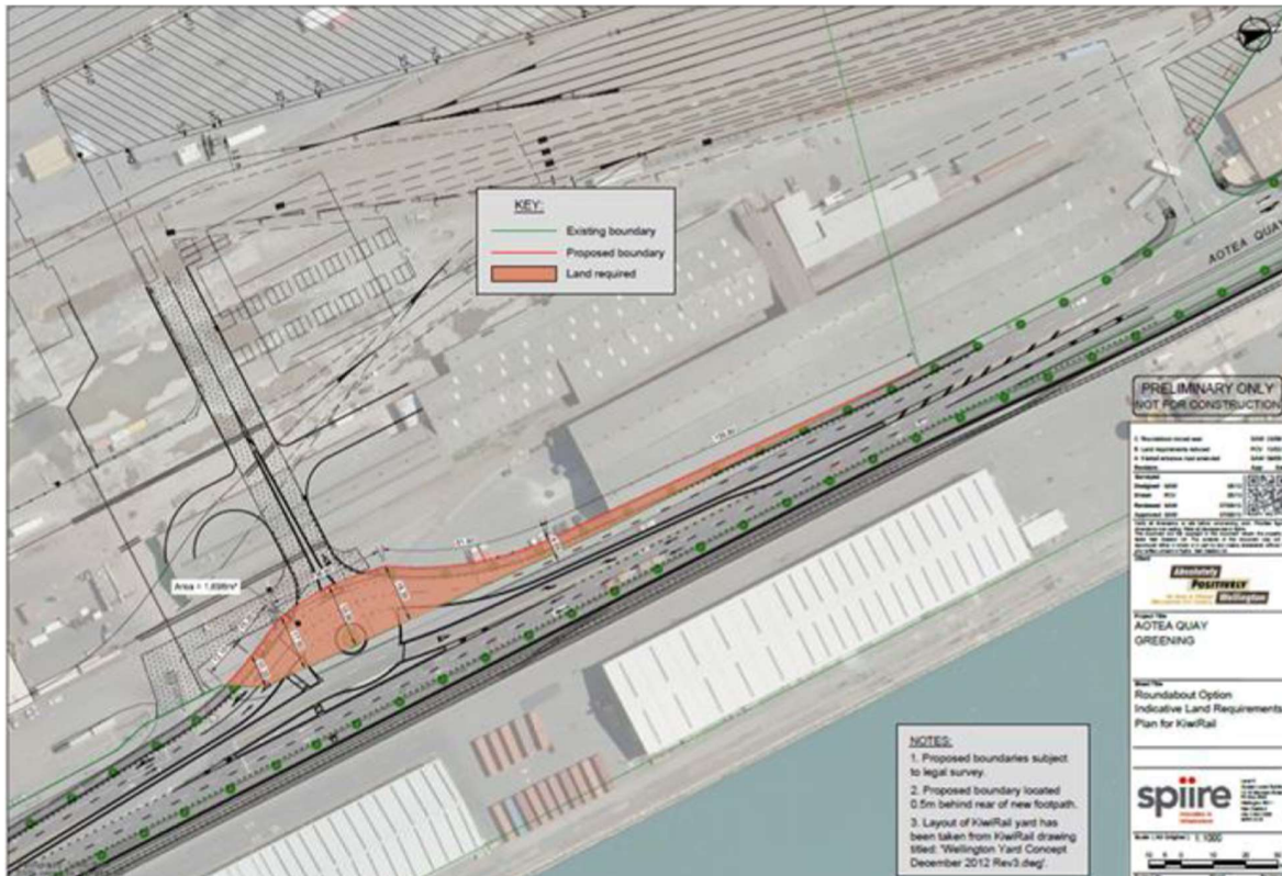
Figure 16: Proposed Layout for Turnaround facility at Aotea Quay
