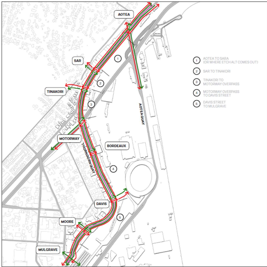
Option 3 - Thorndon Quay Indicative Plan
