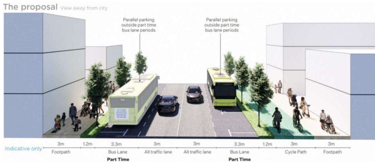
Figure 5: Thorndon Quay Indicative Cross Section
