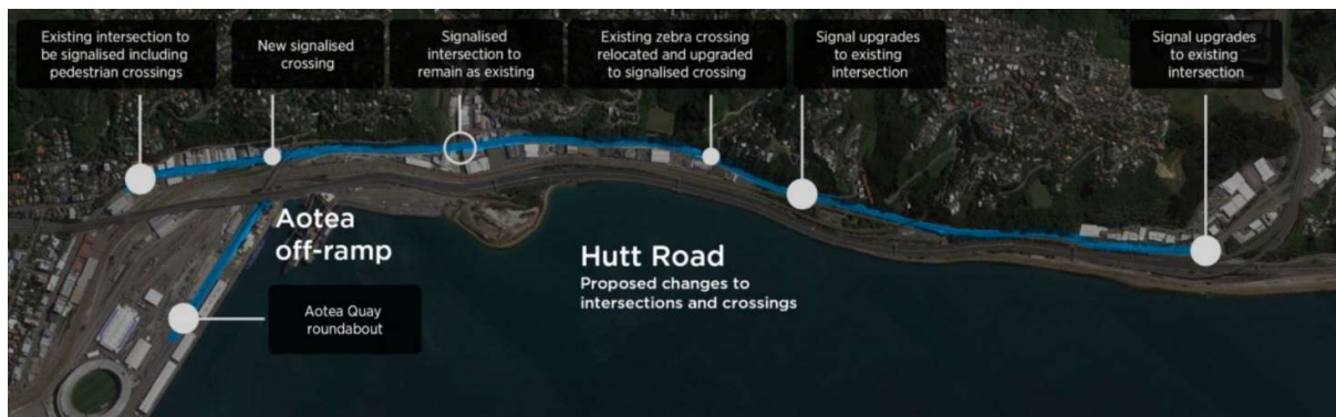
Figure 8: MCA Hutt Road – Proposed Changes to Intersections and Crossings
