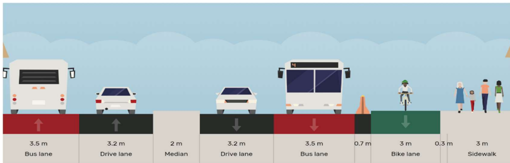
Option 4 - Hutt Road Indicative Cross Section
